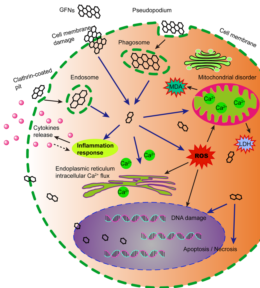
Fig. 3 Schematic diagram showed the possible mechanisms of GFNs cytotoxicity. GFNs get into cells through different ways, which induce in ROS generation, LDH and MDA increase, and \text{Ca}^{2+} release. Subsequently, GFNs cause kinds of cell injury, for instance, cell membrane damage, inflammation, DNA damage, mitochondrial disorders, apoptosis or necrosis
